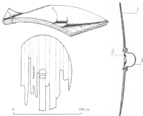
Конструкция римского щита из Дура-Европос ( Bishop M. C., Coulston J. C. N. Roman Military Equipment from the Punic Wars to the fall of Rome. London: Batsford, 1993. P. 151 ):
